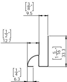
M03C Extended 2 piece J Trim
