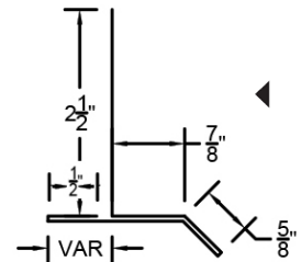
M56C Base flashing
