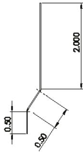
1402 Starter strip
