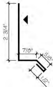
M14C Double L Trim
