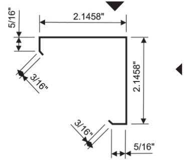
M56C Base flashing
